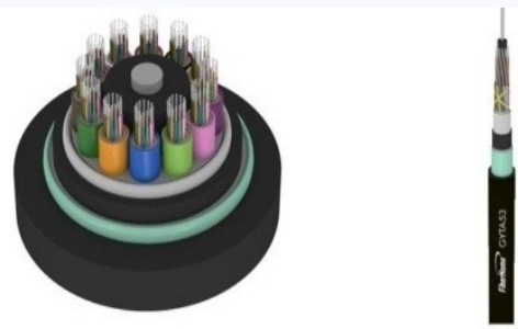
Stranded optical cable
